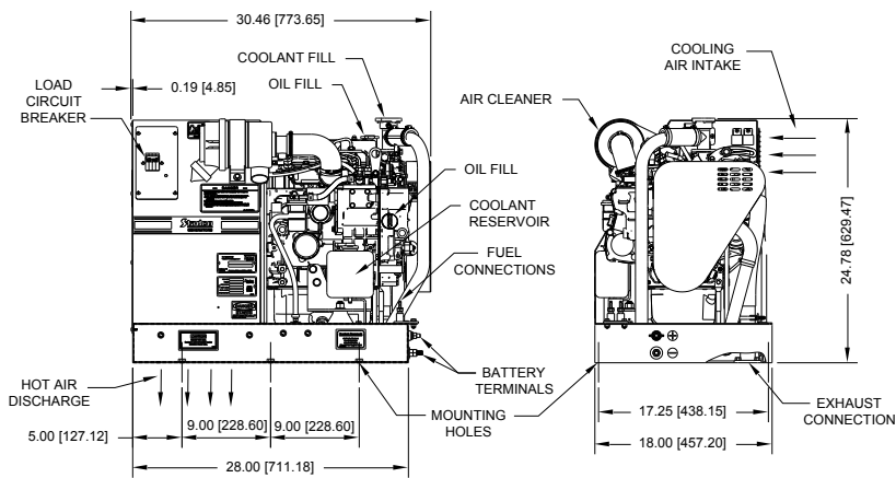
TYPICAL INSTALLATION
